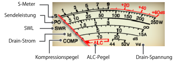
Type 2 (Analog 1 Meter)
