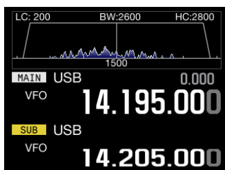
Hauptbandfrequenz & Nebenbandfrequenz Audio Scope & Bandscope-Anzeige
